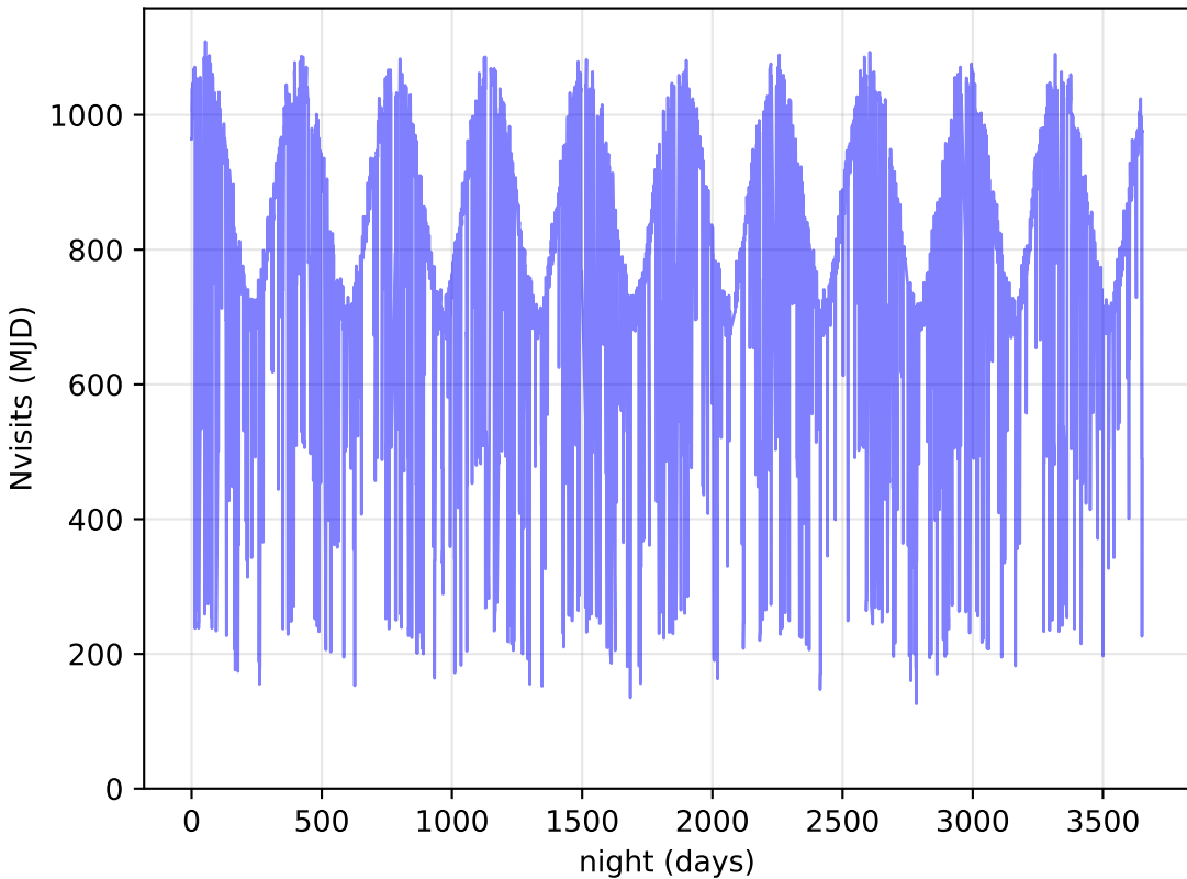
too_10_1v3.4_10yrs All visits: Nvisits
