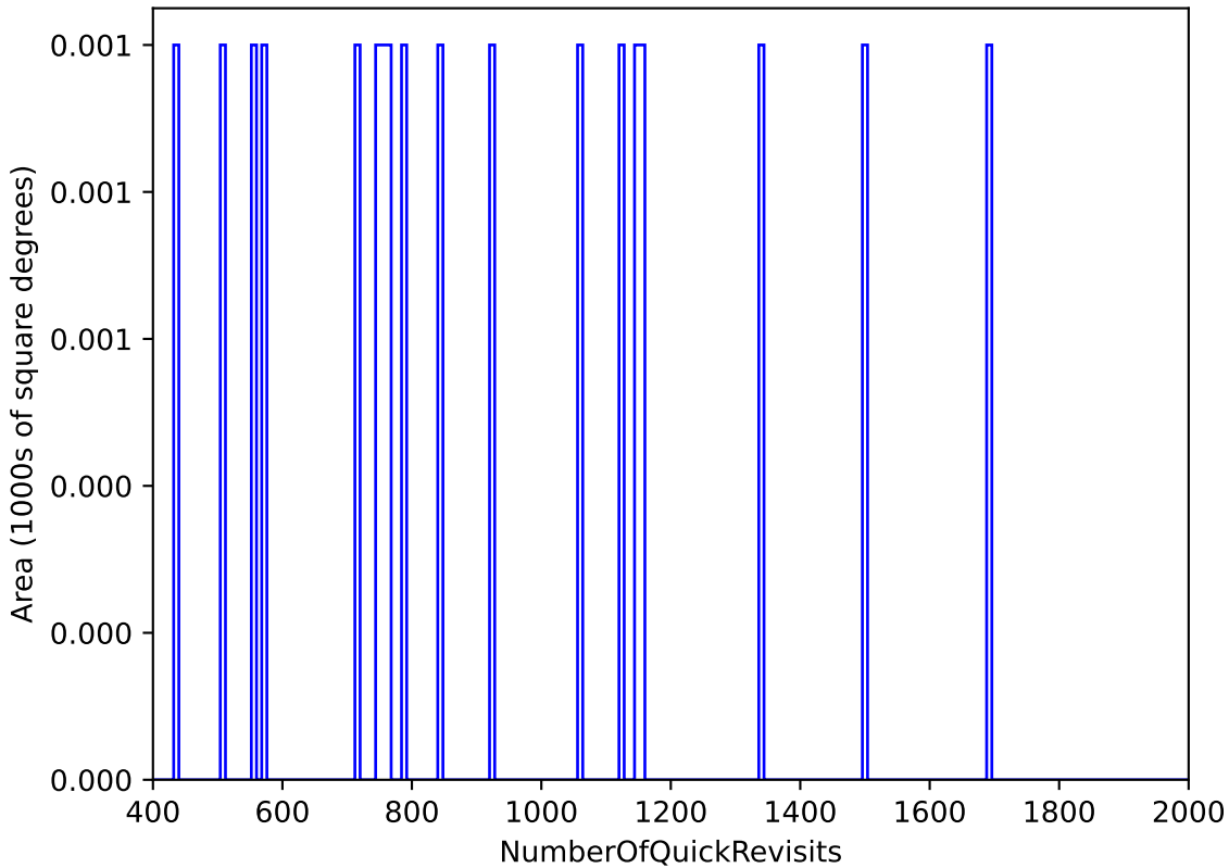
too_10_1v3.4_10yrs WFD: NumberOfQuickRevisits
