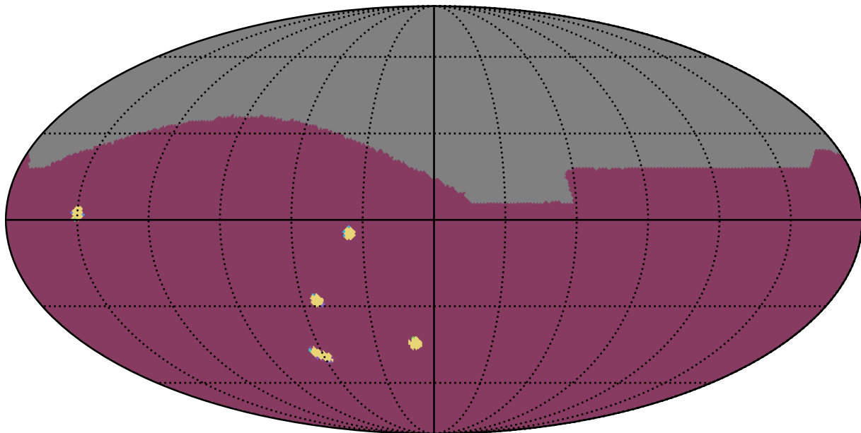
too_10_1v3.4_10yrs All sky: NumberOfQuickRevisits
