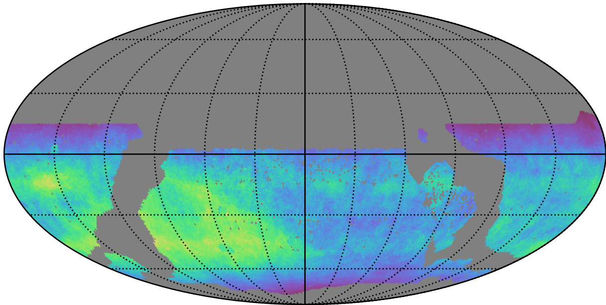
too_10_1v3.4_10yrs WFD z band: Normalized Teff
