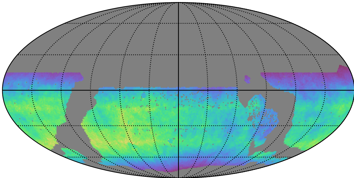
too_10_1v3.4_10yrs WFD y band: Normalized Teff
