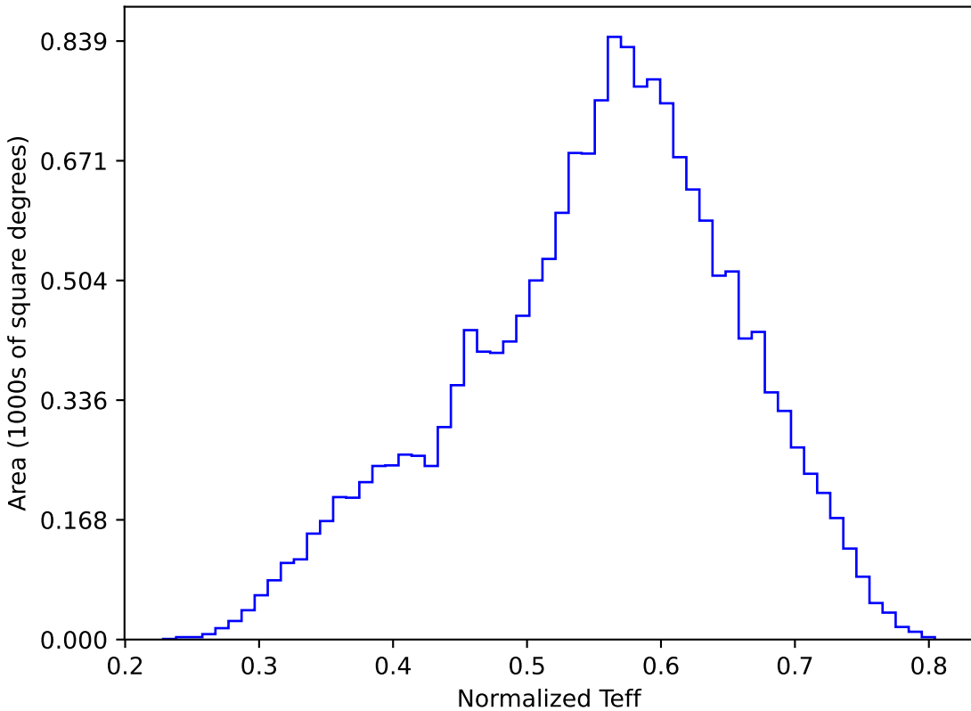
too_10_1v3.4_10yrs WFD y band: Normalized Teff
