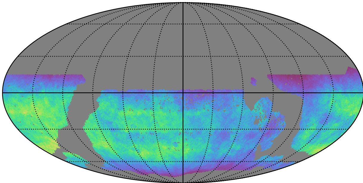
too_10_1v3.4_10yrs WFD u band: Normalized Teff
