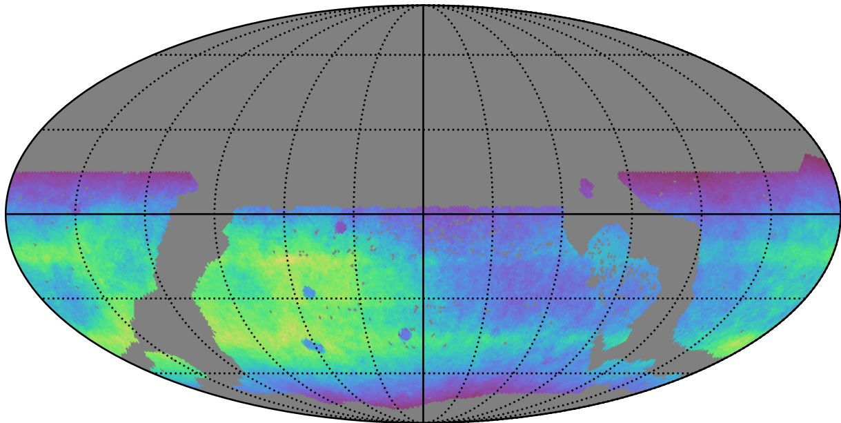
too_10_1v3.4_10yrs WFD r band: Normalized Teff
