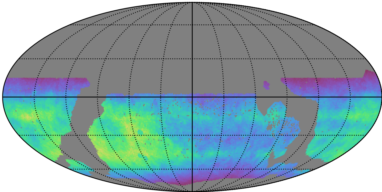
too_10_1v3.4_10yrs WFD i band: Normalized Teff
