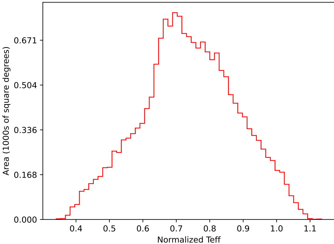
too_10_1v3.4_10yrs WFD i band: Normalized Teff
