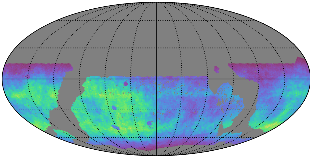
too_10_1v3.4_10yrs WFD g band: Normalized Teff
