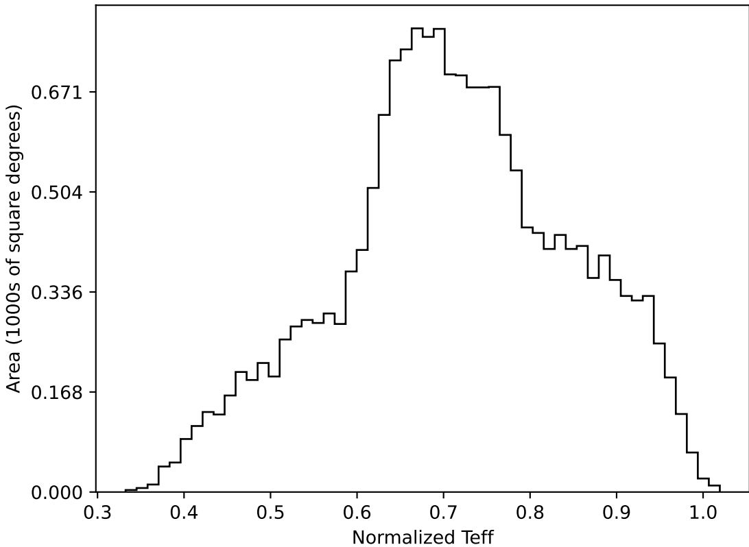
too_10_1v3.4_10yrs WFD all bands: Normalized Teff
