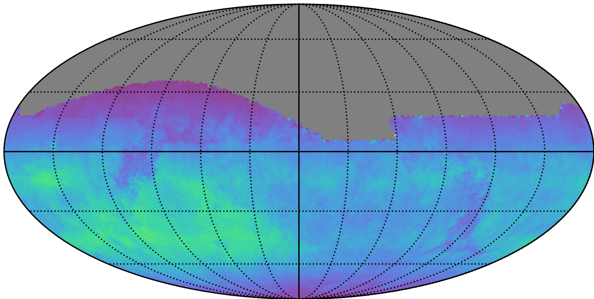
too_10_1v3.4_10yrs All sky z band: Normalized Teff
