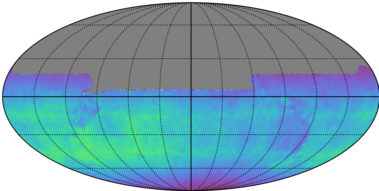
too_10_1v3.4_10yrs All sky y band: Normalized Teff
