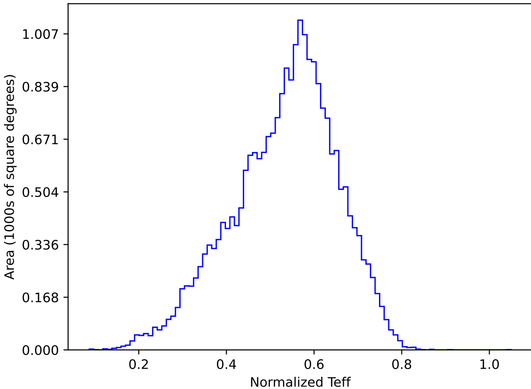
too_10_1v3.4_10yrs All sky y band: Normalized Teff
