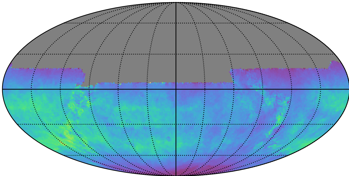
too_10_1v3.4_10yrs All sky u band: Normalized Teff
