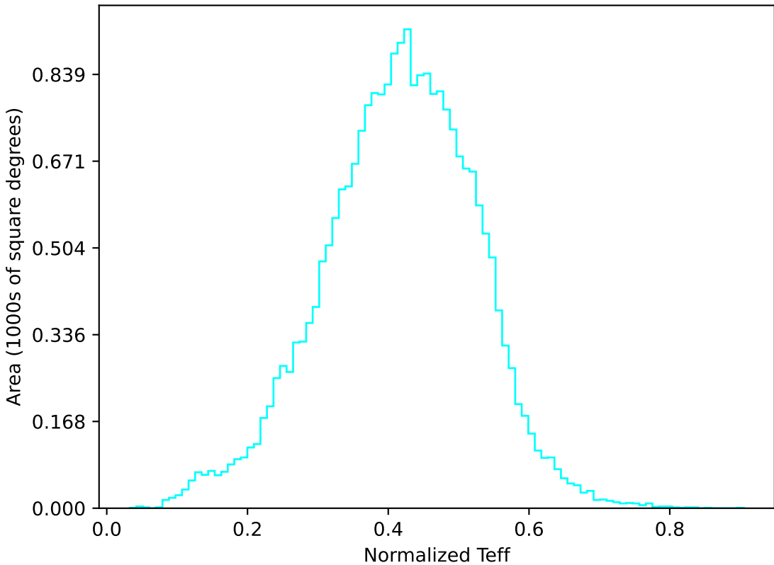
too_10_1v3.4_10yrs All sky u band: Normalized Teff
