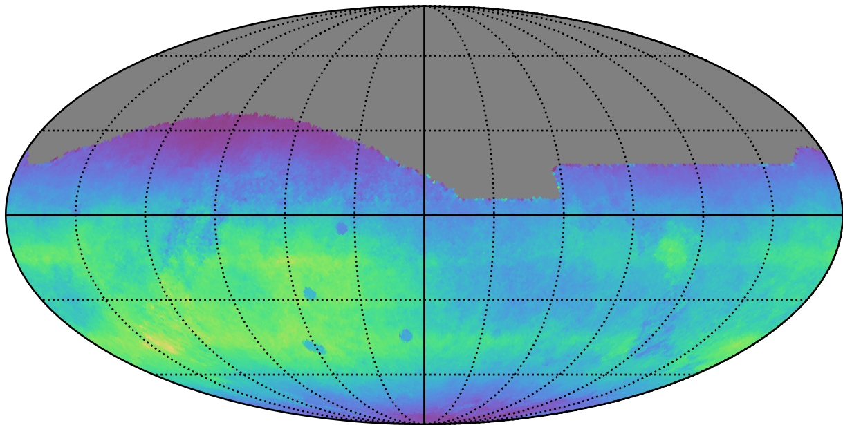
too_10_1v3.4_10yrs All sky r band: Normalized Teff
