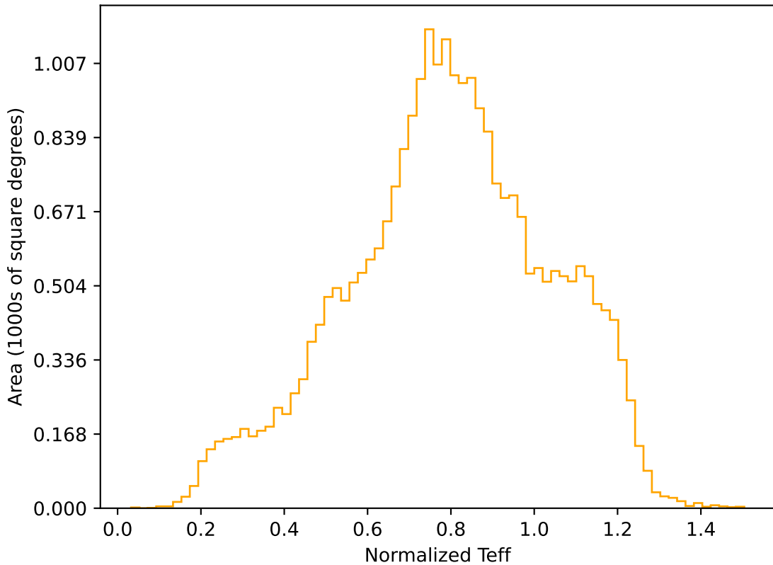
too_10_1v3.4_10yrs All sky r band: Normalized Teff
