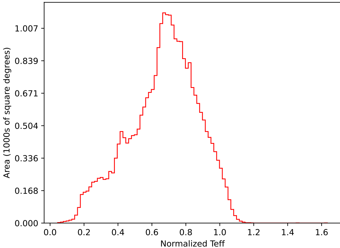
too_10_1v3.4_10yrs All sky i band: Normalized Teff
