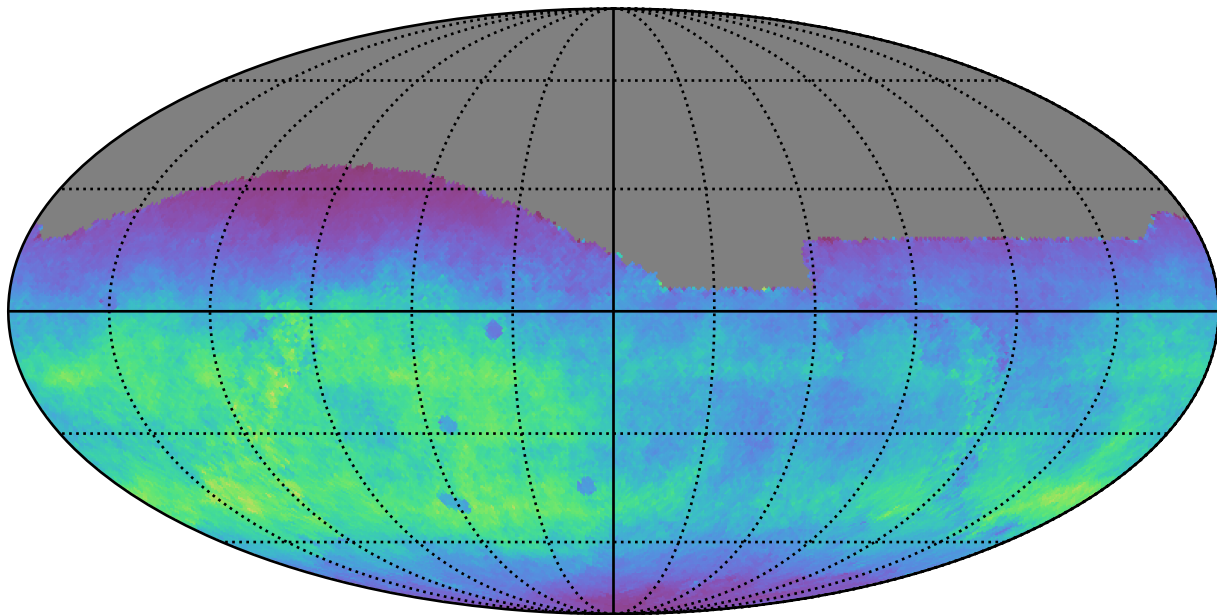
too_10_1v3.4_10yrs All sky g band: Normalized Teff
