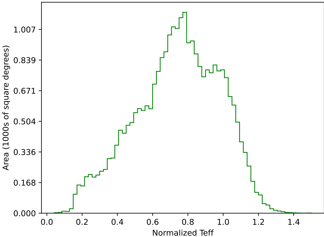
too_10_1v3.4_10yrs All sky g band: Normalized Teff
