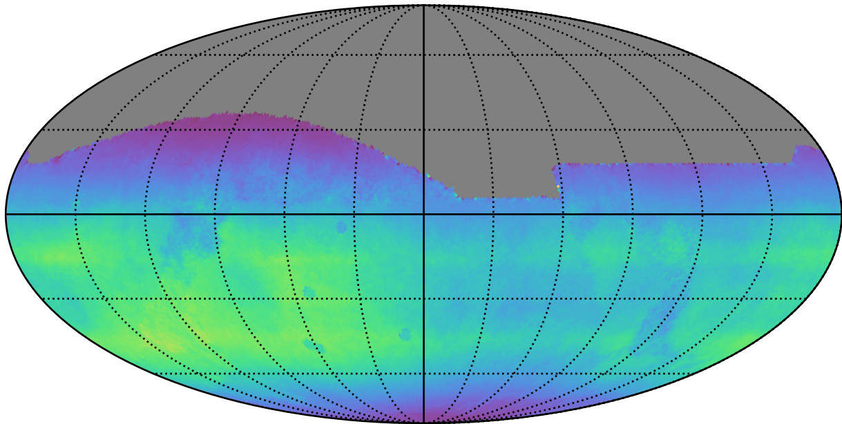
too_10_1v3.4_10yrs All sky all bands: Normalized Teff
