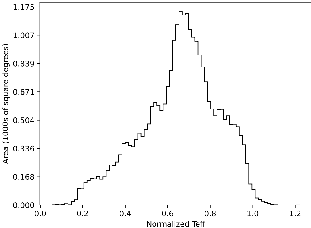
too_10_1v3.4_10yrs All sky all bands: Normalized Teff
