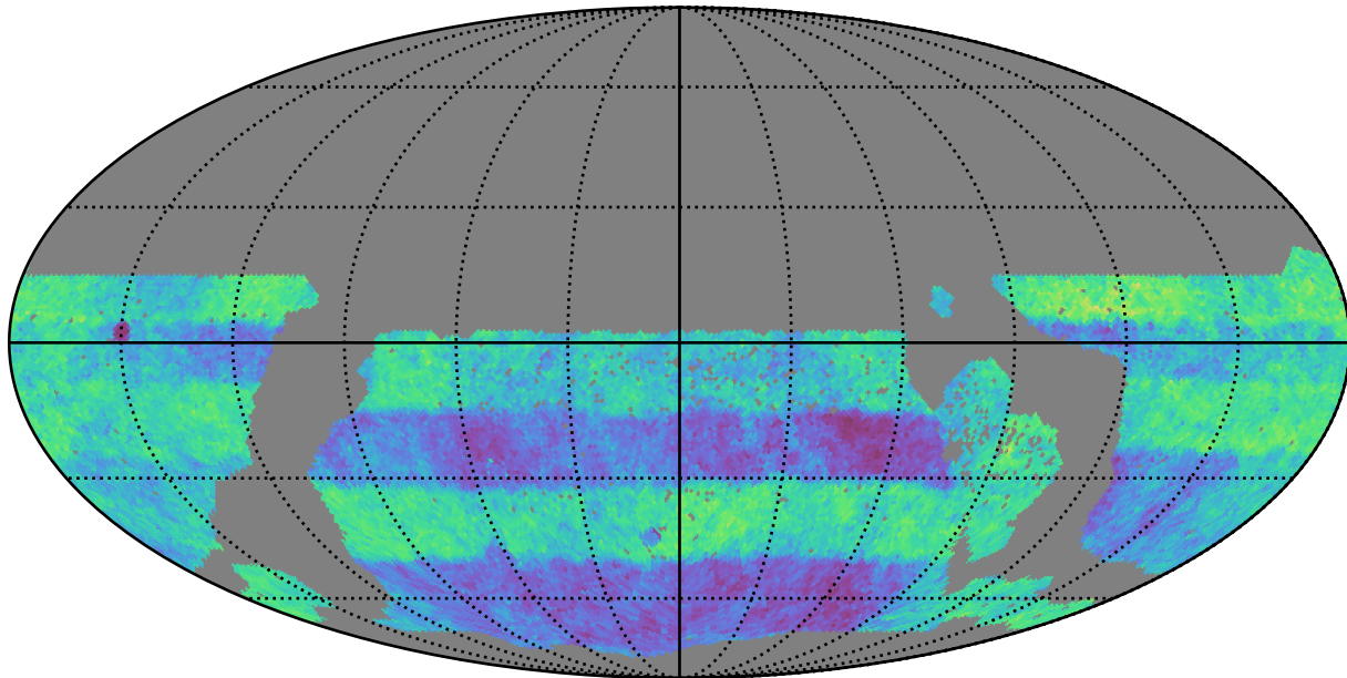
too_10_1v3.4_10yrs WFD: Normalized Proper Motion Uncert @ 24.0
