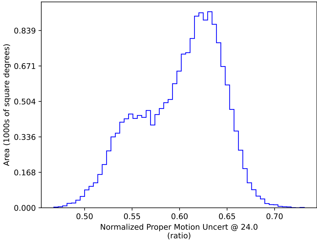
too_10_1v3.4_10yrs WFD: Normalized Proper Motion Uncert @ 24.0
