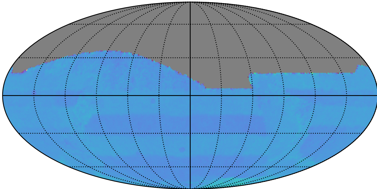
too_10_1v3.4_10yrs All sky: Normalized Proper Motion Uncert @ 20.5
