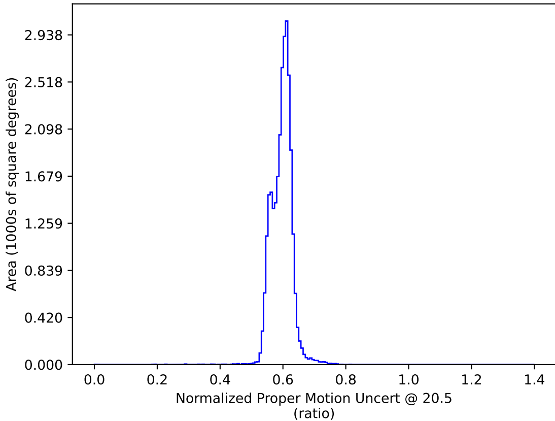
too_10_1v3.4_10yrs All sky: Normalized Proper Motion Uncert @ 20.5
