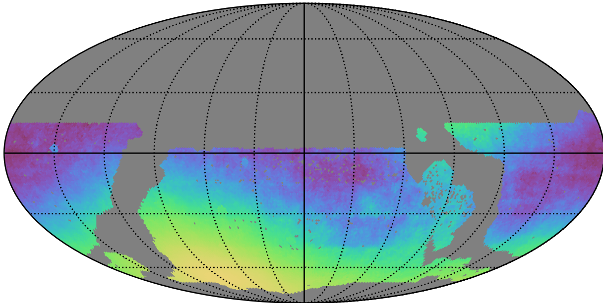
too_10_1v3.4_10yrs WFD: Normalized Parallax Uncert @ 24.0
