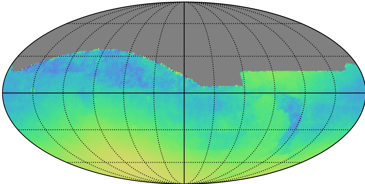
too_10_1v3.4_10yrs All sky: Normalized Parallax Uncert @ 24.0
