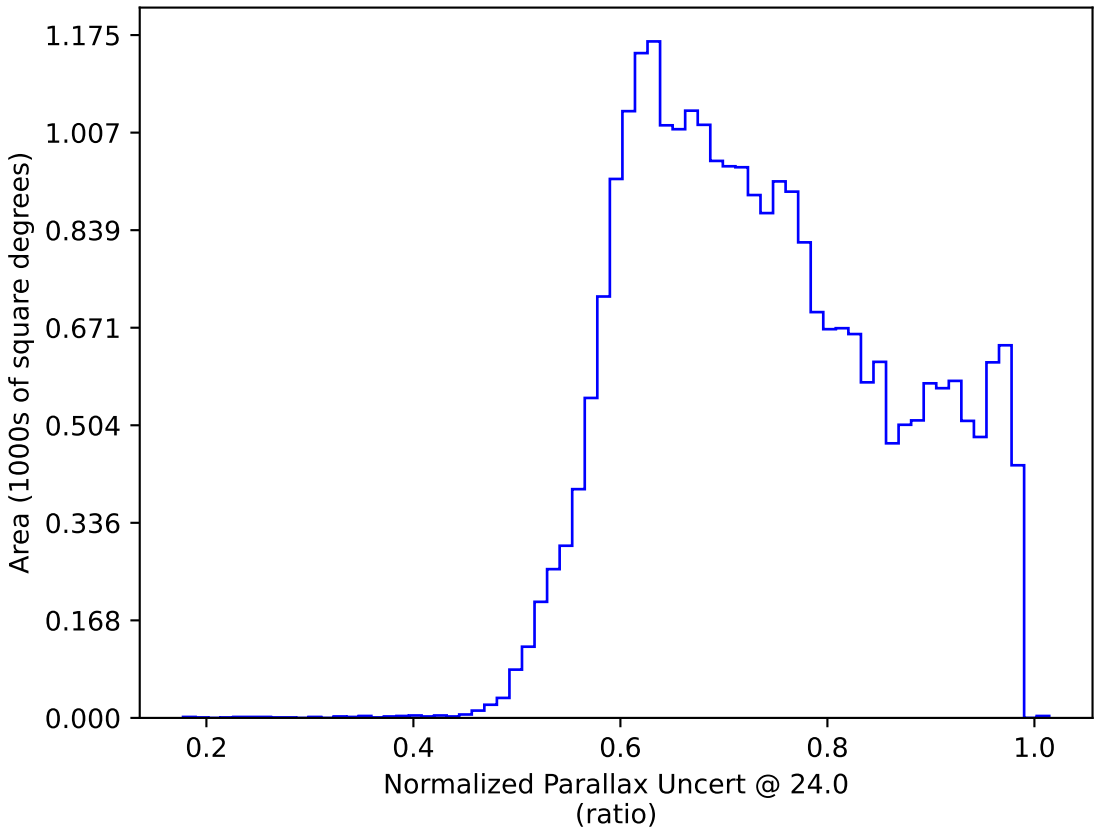
too_10_1v3.4_10yrs All sky: Normalized Parallax Uncert @ 24.0
