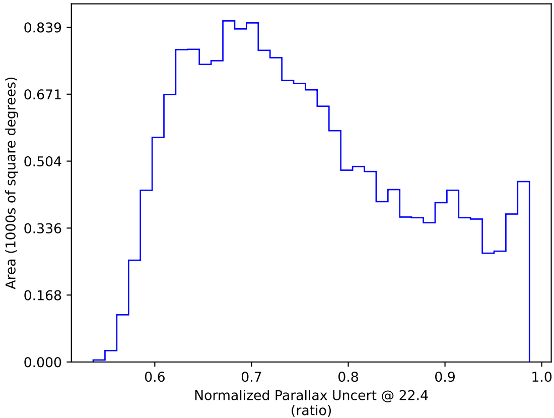
too_10_1v3.4_10yrs WFD: Normalized Parallax Uncert @ 22.4
