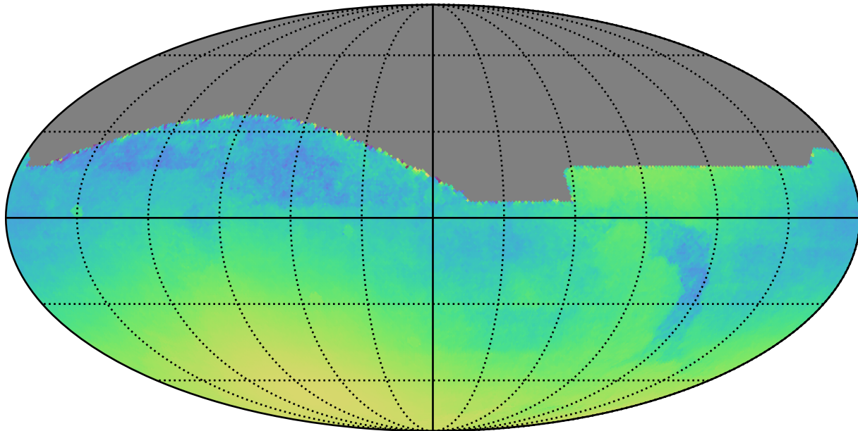
too_10_1v3.4_10yrs All sky: Normalized Parallax Uncert @ 22.4
