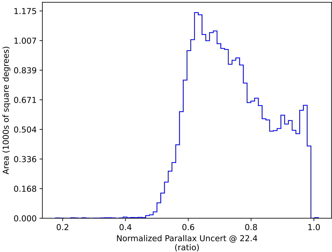
too_10_1v3.4_10yrs All sky: Normalized Parallax Uncert @ 22.4
