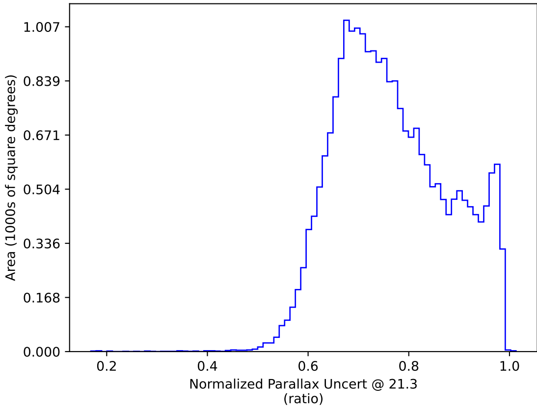
too_10_1v3.4_10yrs All sky y band only: Normalized Parallax Uncert @ 21.3
