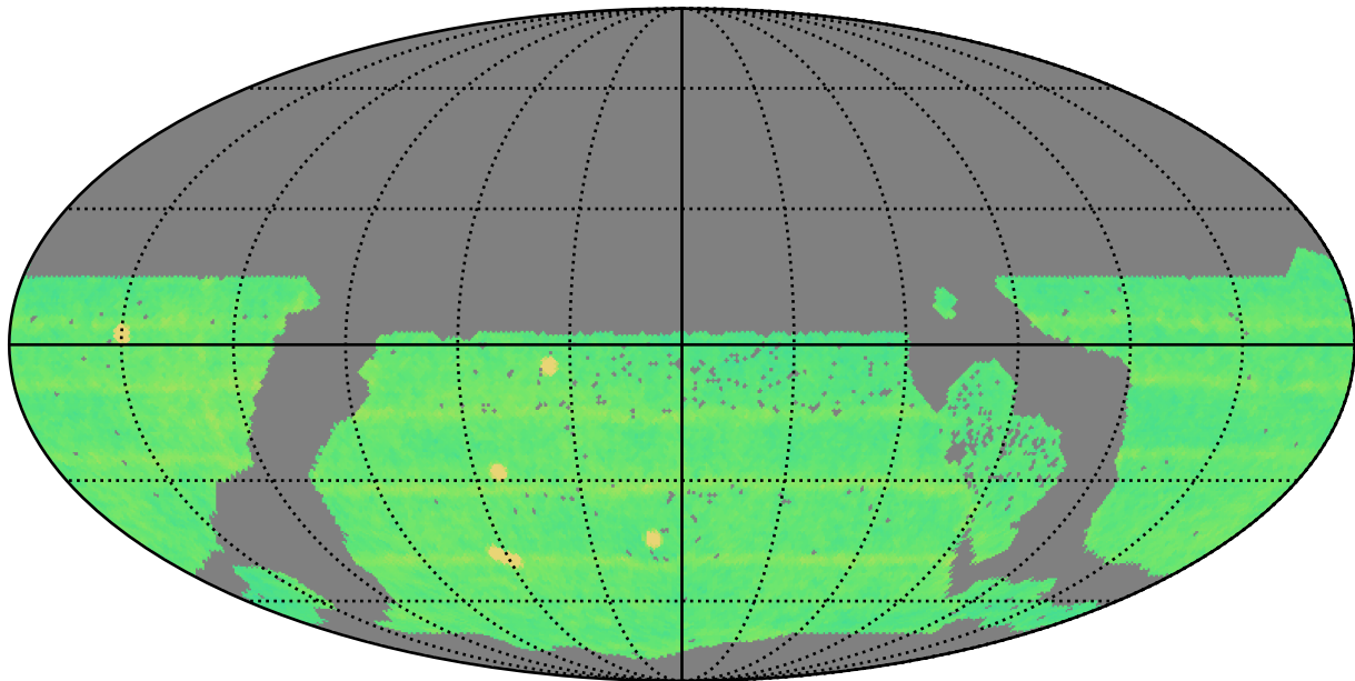
too_10_1v3.4_10yrs WFD all bands: N Unique Nights
