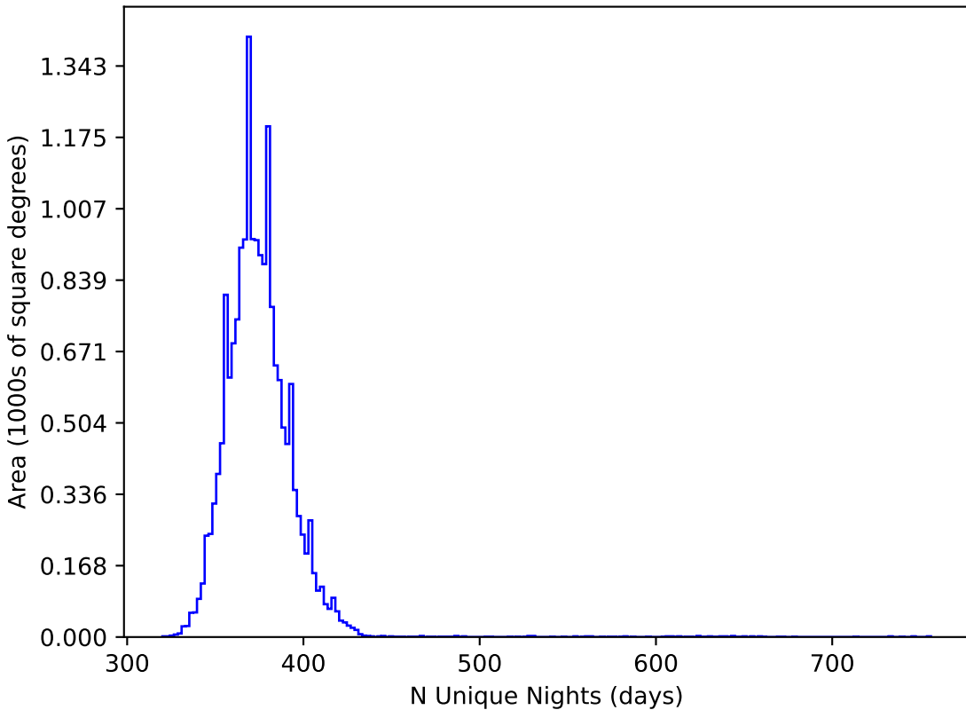
too_10_1v3.4_10yrs WFD all bands: N Unique Nights
