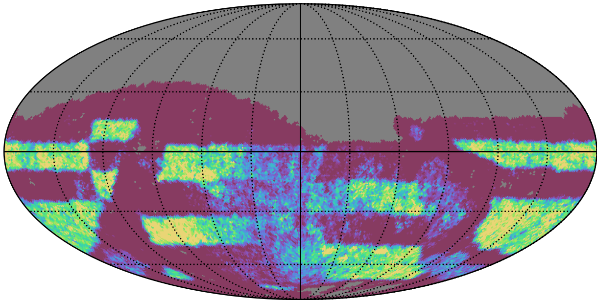
too_10_1v3.4_10yrs Yr 3-4 z band: NVisits
