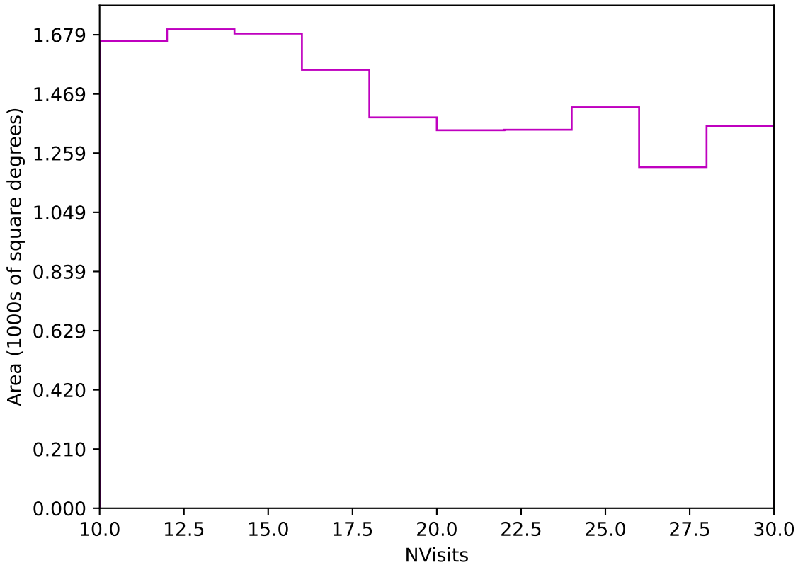
too_10_1v3.4_10yrs Yr 3-4 z band: NVisits
