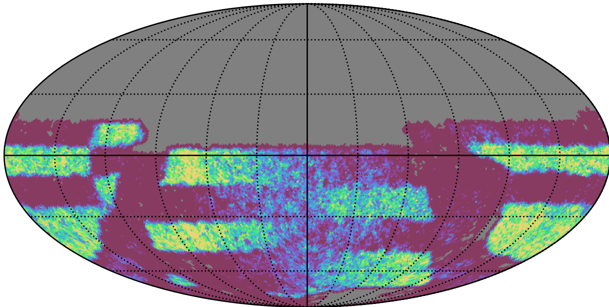
too_10_1v3.4_10yrs Yr 3-4 y band: NVisits
