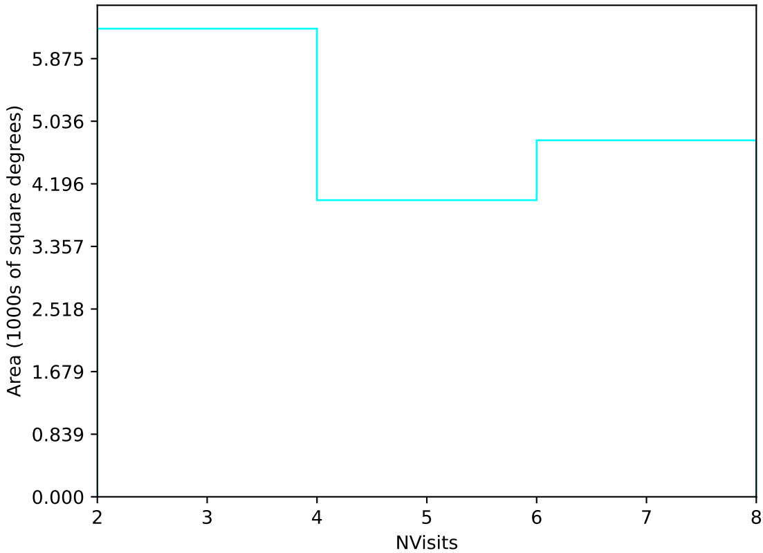
too_10_1v3.4_10yrs Yr 3-4 u band: NVisits
