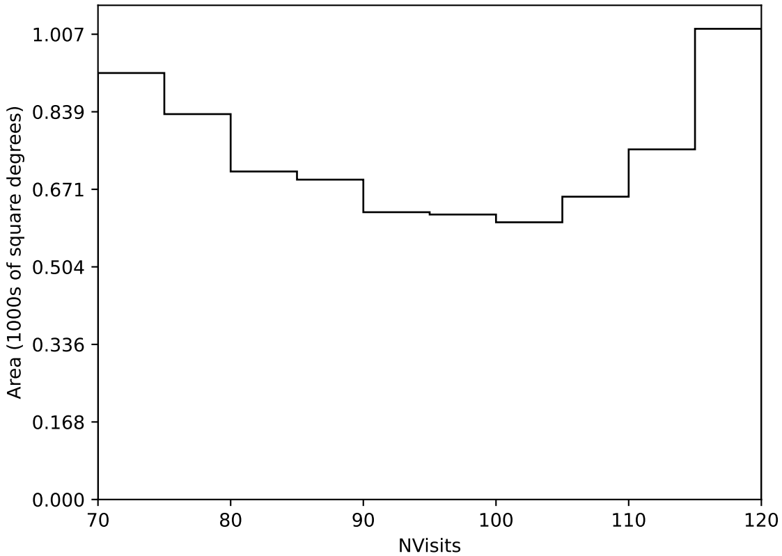
too_10_1v3.4_10yrs Yr 3-4 all bands: NVisits
