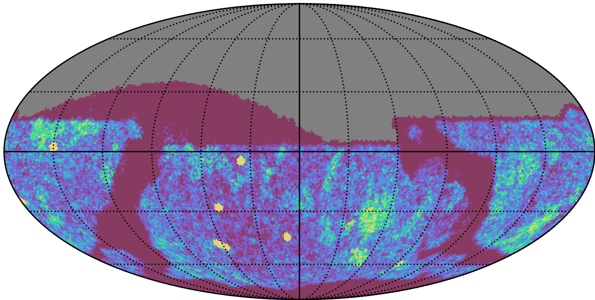
too_10_1v3.4_10yrs Yr 1 z band: NVisits
