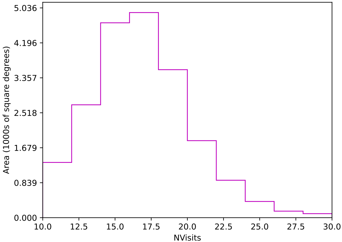
too_10_1v3.4_10yrs Yr 1 z band: NVisits
