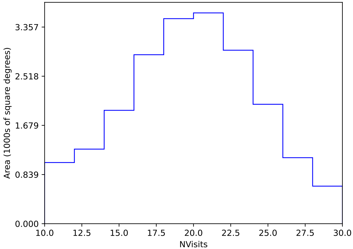
too_10_1v3.4_10yrs Yr 1 y band: NVisits
