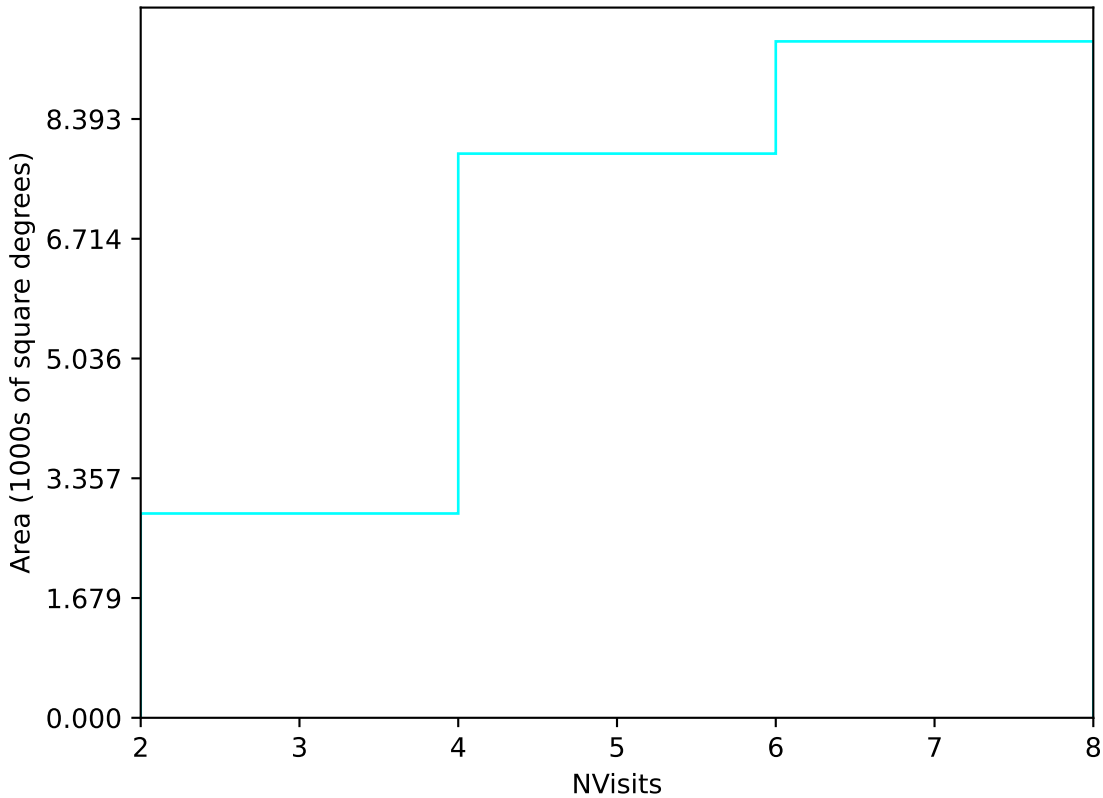
too_10_1v3.4_10yrs Yr 1 u band: NVisits
