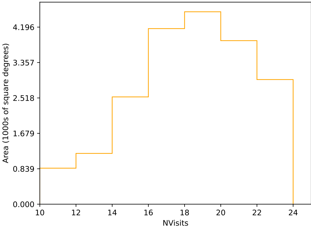
too_10_1v3.4_10yrs Yr 1 r band: NVisits
