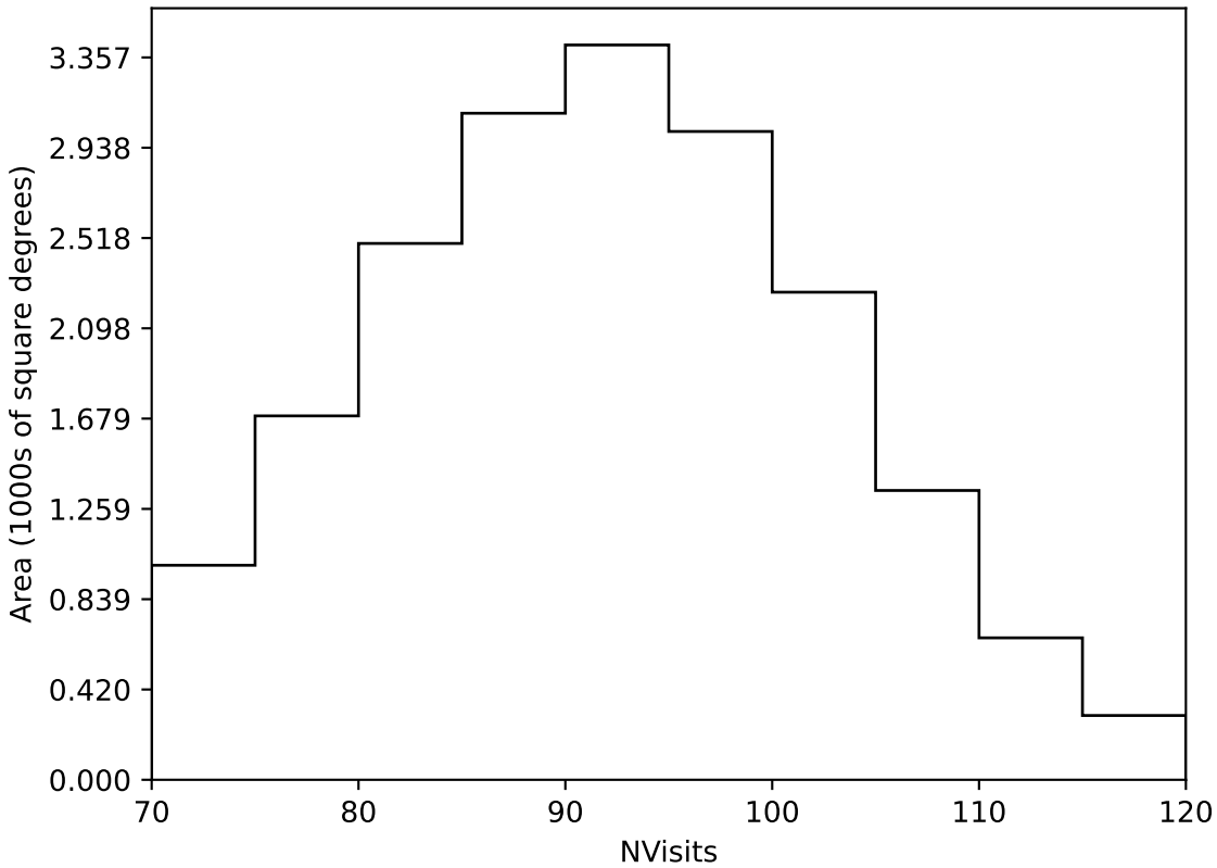
too_10_1v3.4_10yrs Yr 1 all bands: NVisits
