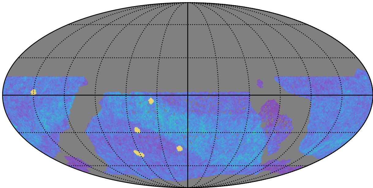
too_10_1v3.4_10yrs WFD z band: NVisits
