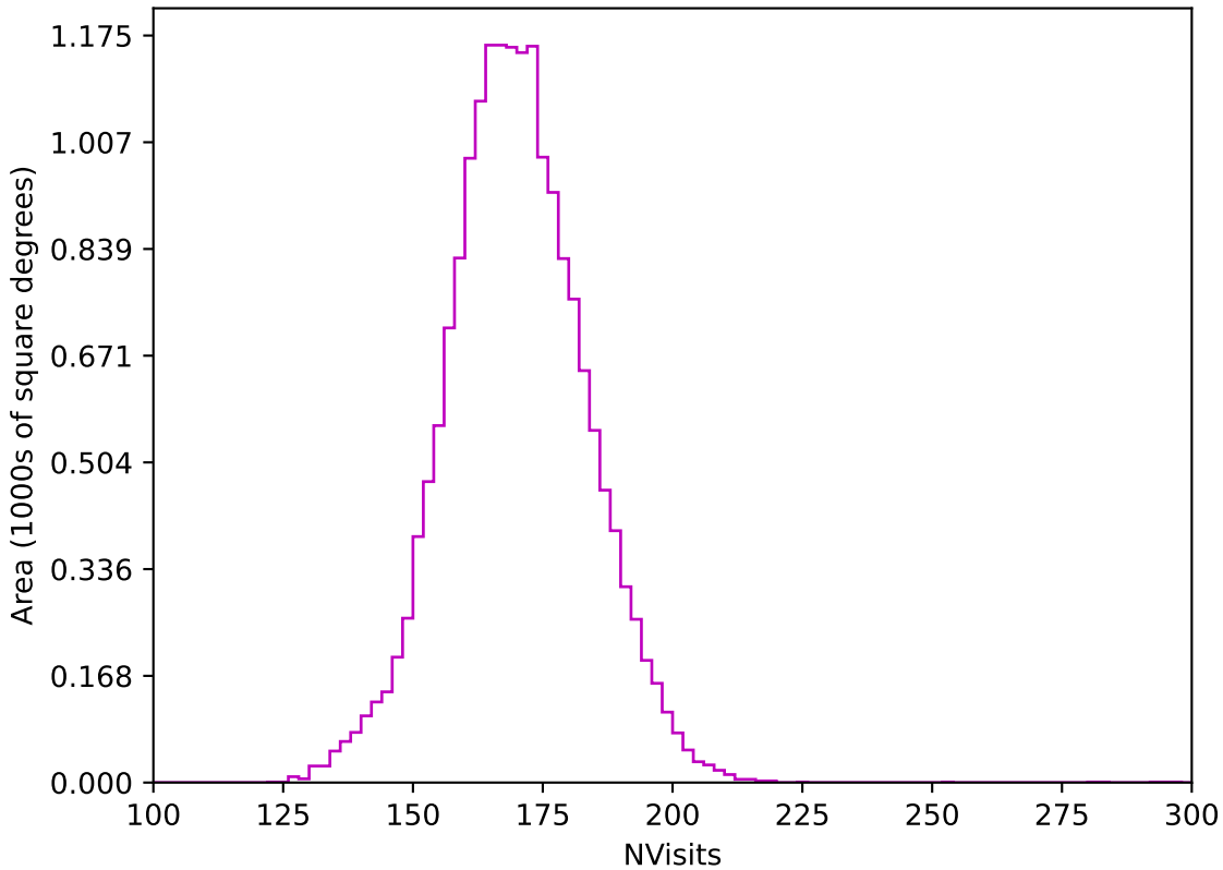
too_10_1v3.4_10yrs WFD z band: NVisits
